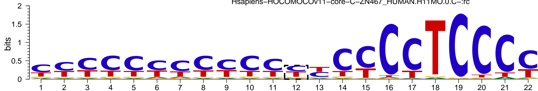
Hsapiens-HOCOMOCov11-core-C-WT1_HUMAN.H11MO.0.C-:rc
