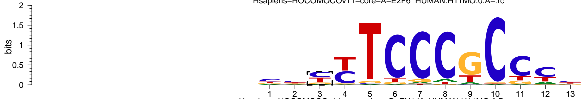
Hsapiens-HOCOMOCov11-secondary-D-ZN148_HUMAN.H11MO.0.D-:rc
