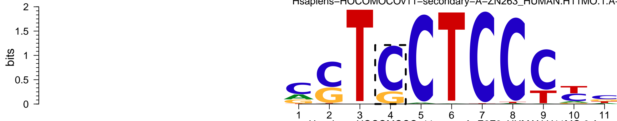
Hsapiens-HOCOMOCov11-core-A-E2F6_HUMAN.H11MO.0.A-:rc
