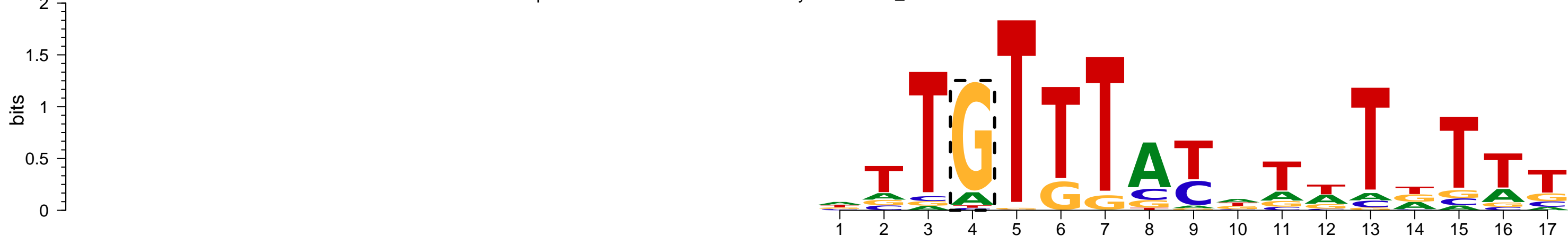
Hsapiens-HOCOMOCov11-core-C-FOXO4_HUMAN.H11MO.0.C
