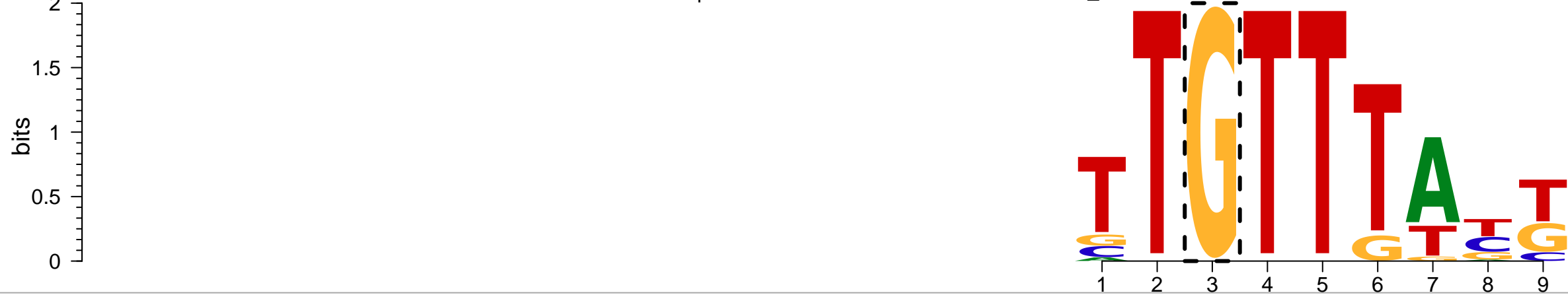
Hsapiens-HOCOMOCov11-core-C-FOXO4_HUMAN.H11MO.0.C
