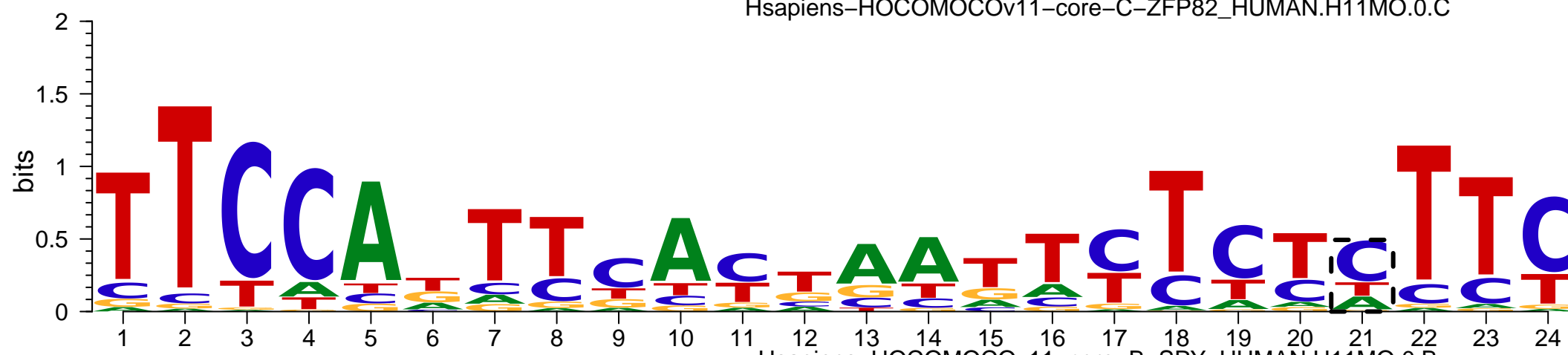
Hsapiens-HOCOMOCov11-core-B-SRY_HUMAN.H11MO.0.B
