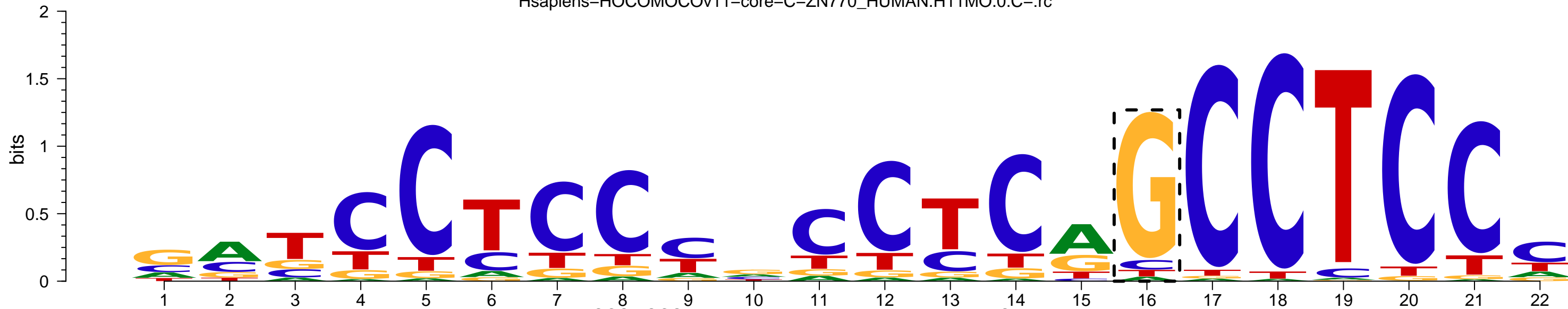
Hsapiens-HOCOMOCov11-secondary-D-AP2D_HUMAN.H11MO.0.D-:rc
