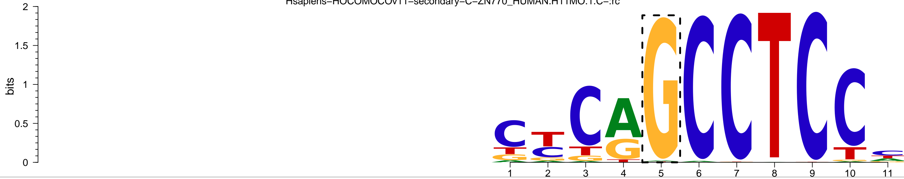
Hsapiens-HOCOMOCov11-secondary-C-ZN770_HUMAN.H11MO.1.C-:rc
