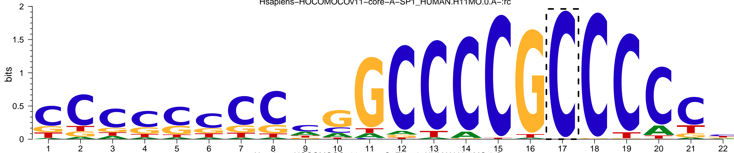
Hsapiens-HOCOMOCov11-core-C-ZN770_HUMAN.H11MO.0.C-:rc
