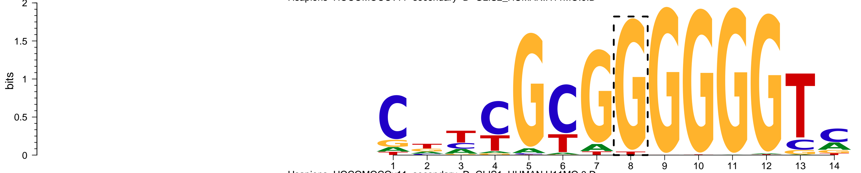
Hsapiens-HOCOMOCov11-secondary-D-GLIS1_HUMAN.H11MO.0.D
