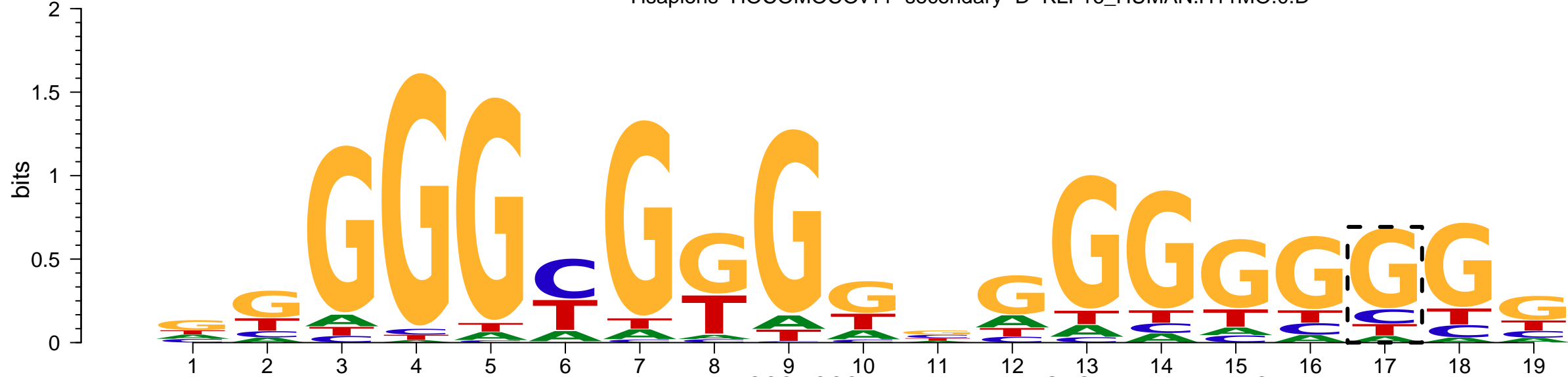
Hsapiens-HOCOMOCov11-secondary-D-GLIS2_HUMAN.H11MO.0.D
