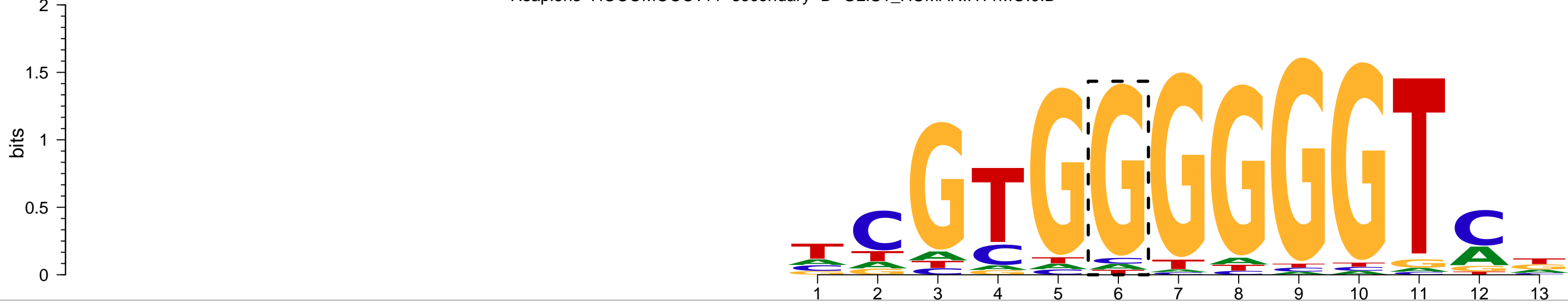
Hsapiens-HOCOMOCov11-secondary-D-GLIS1_HUMAN.H11MO.0.D
