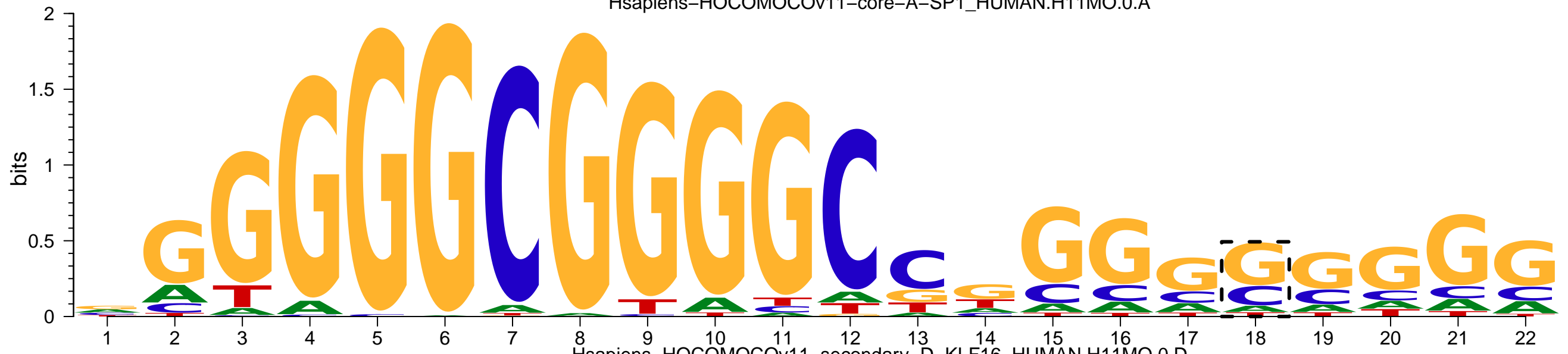
Hsapiens-HOCOMOCov11-secondary-D-KLF16_HUMAN.H11MO.0.D
